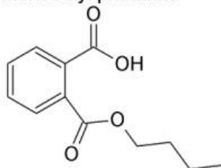
Monobutyl phthalate
