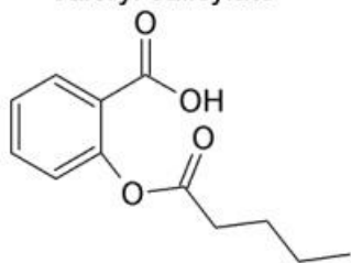
Valeryl salicylate
